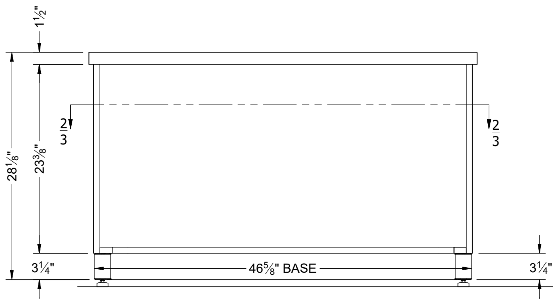
3 3 BACK VIEW
